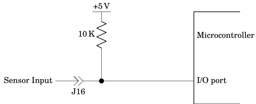
Figure 8.2: Sensor Input Circuit
