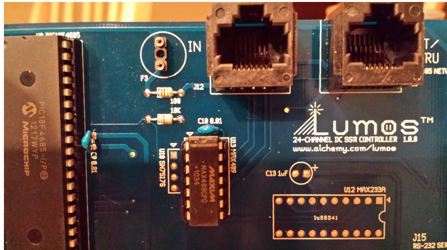
Figure 7.1: Lumos Board with Full-Duplex RS-485 Option
