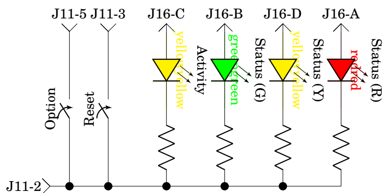
Figure 10.1: Example of a Front Panel Circuit for a Lumos Board
