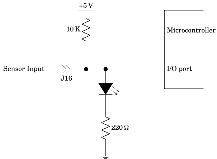
Figure 8.3: Sensor Input Circuit with LED Present
