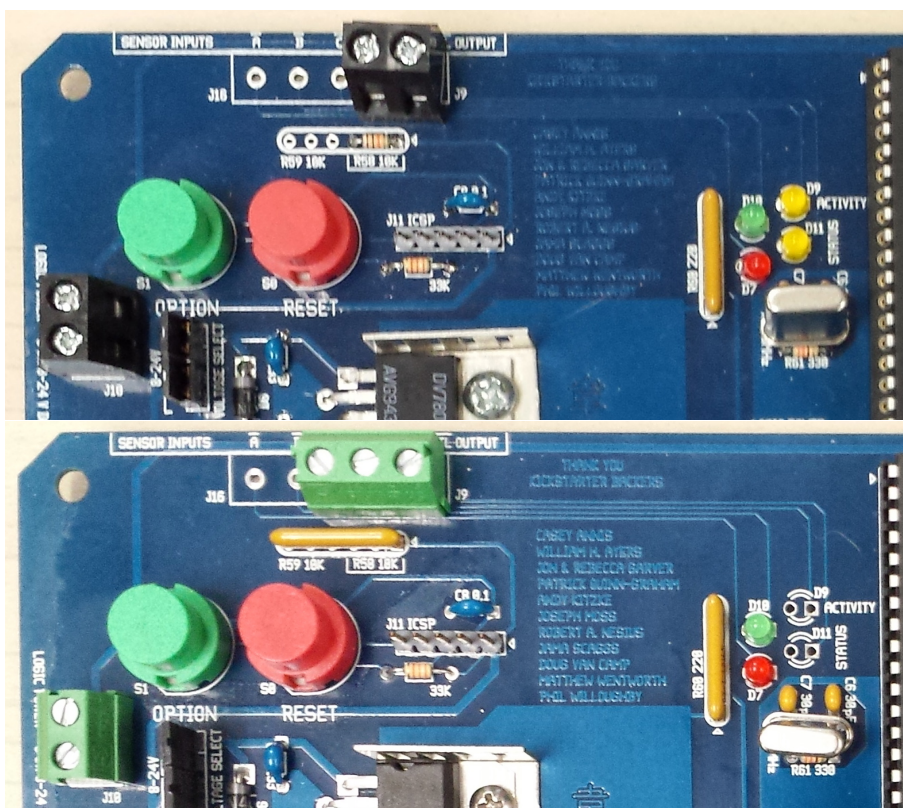
Figure 8.1: Board with No Sensors (above) and Two Sensors (below)
