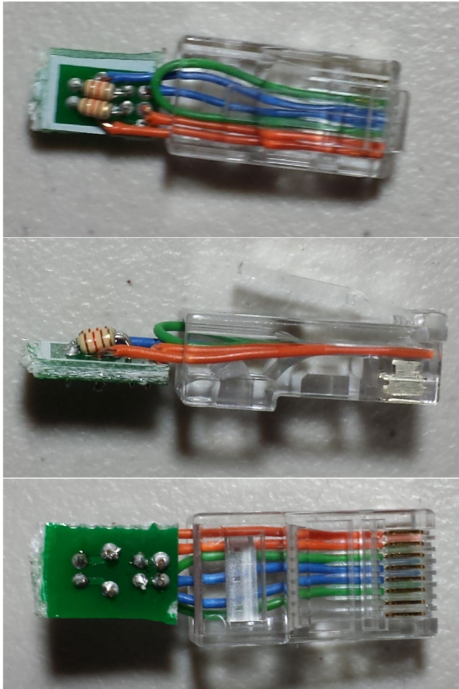
Figure 7.4: Fully Wired Terminator
