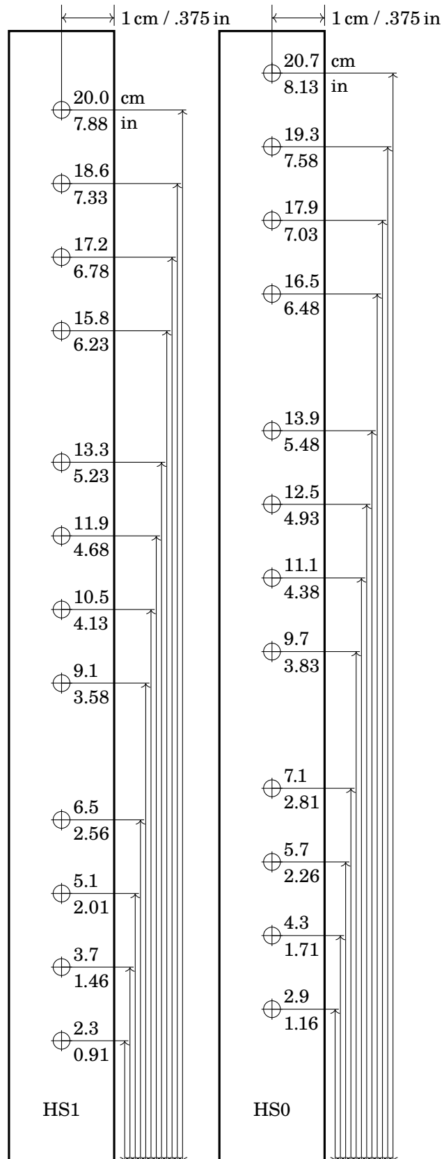
Figure 4.1: Drill Locations for Heat Sinks HS0–HS1
