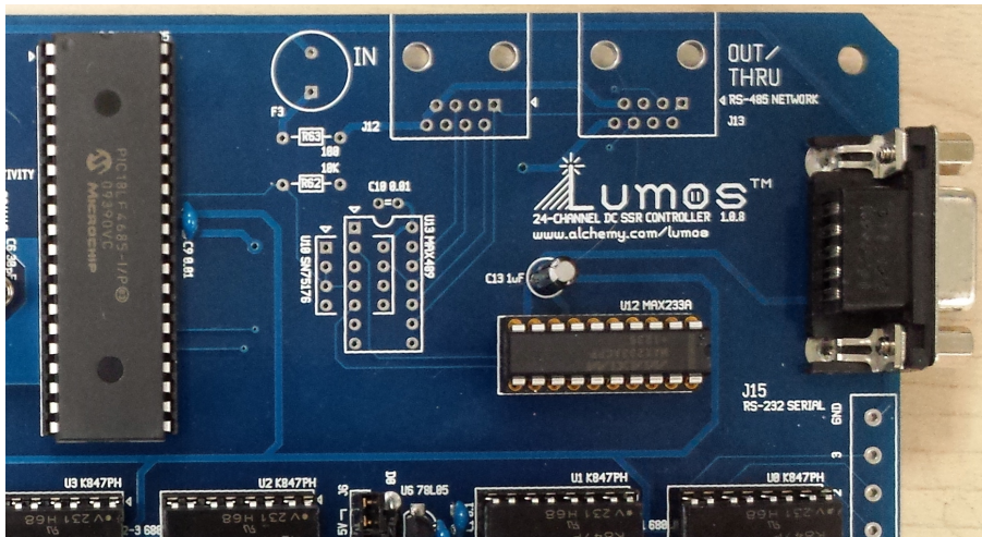
Figure 7.5: Lumos Board with RS-232 Option
