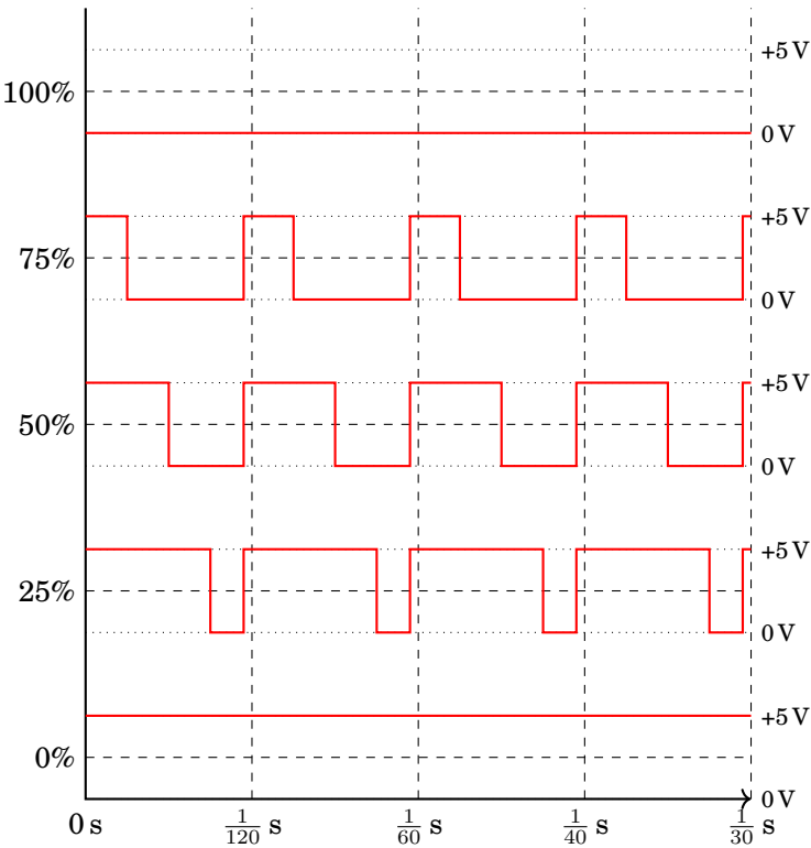
Figure A.1: Duty Cycles of Channel Logic Drive Outputs
