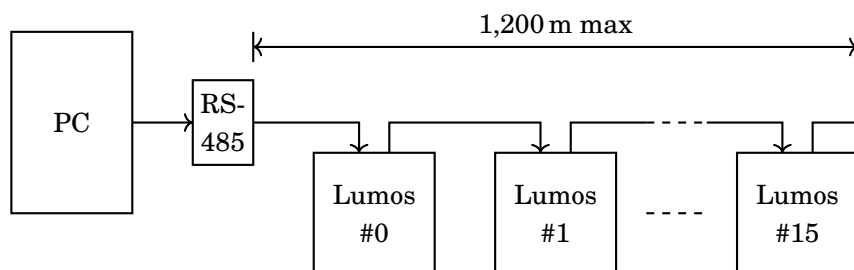
Figure 4.2: Network Connection Diagram
