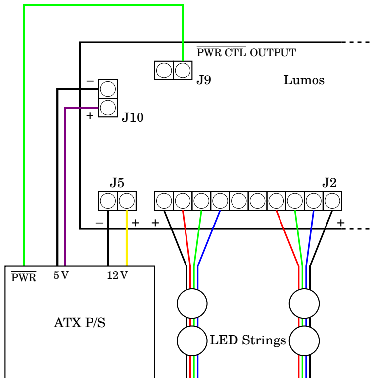
Figure 4.4: Example Wiring of Two 12 V RGB LED Strings
