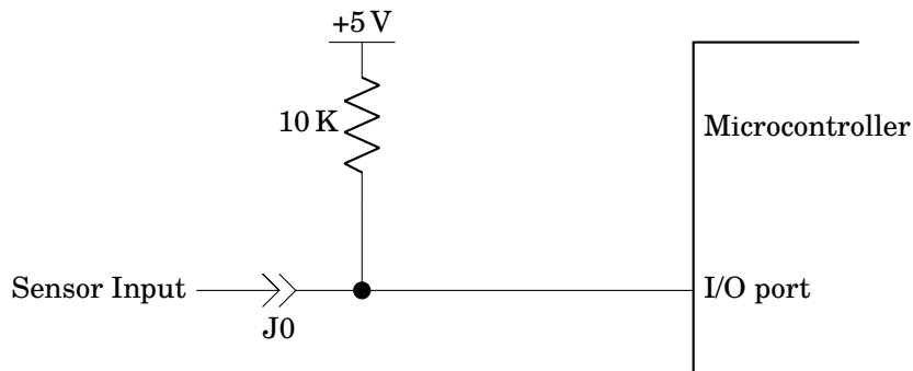
Figure 7.1: Sensor Input Circuit
