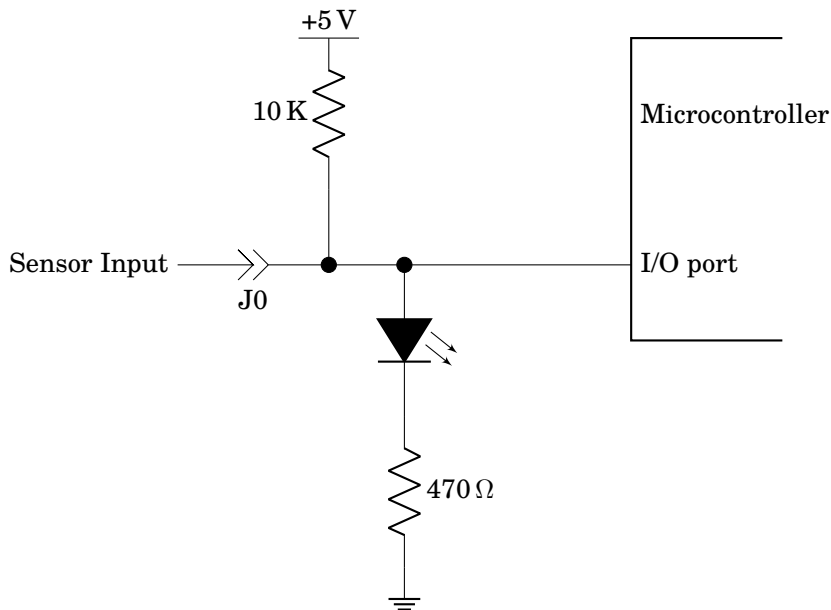
Figure 7.2: Sensor Input Circuit with LED Present
