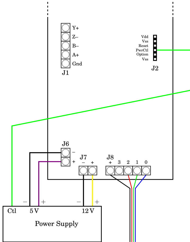
Figure 4.3: Example Wiring of a 12 V RGB LED String
