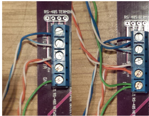
Figure 4.2: Connected Network Cables: Single (left), Daisy-Chained (right)
