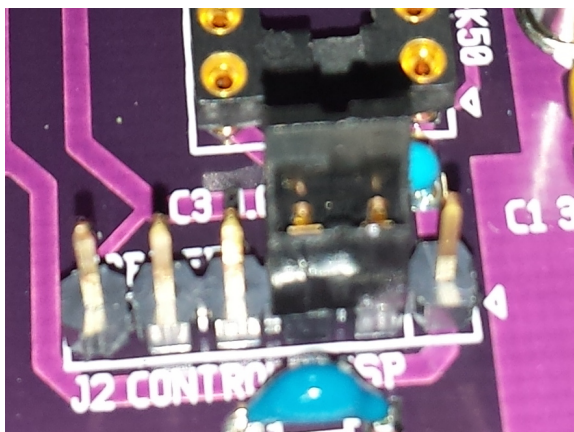
Figure 4.1: Resetting a 4-Channel DC Lumos Board Via Jumper on J2-2 and J2-3
