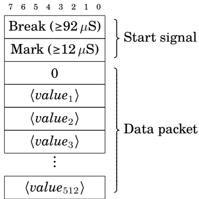
Figure 8.1: DMX Packet
