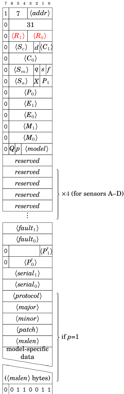
Figure 7.2: 0x71f [reply] Query Response from Lumos Controller
