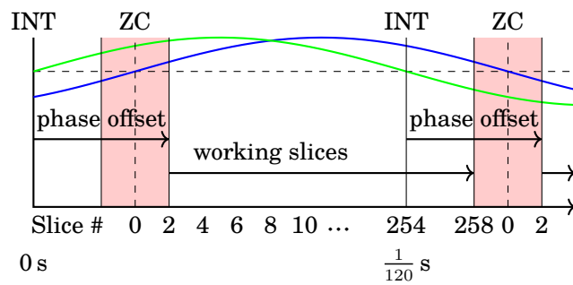
Figure 9.5: Cycle Timing with Phase Offset
